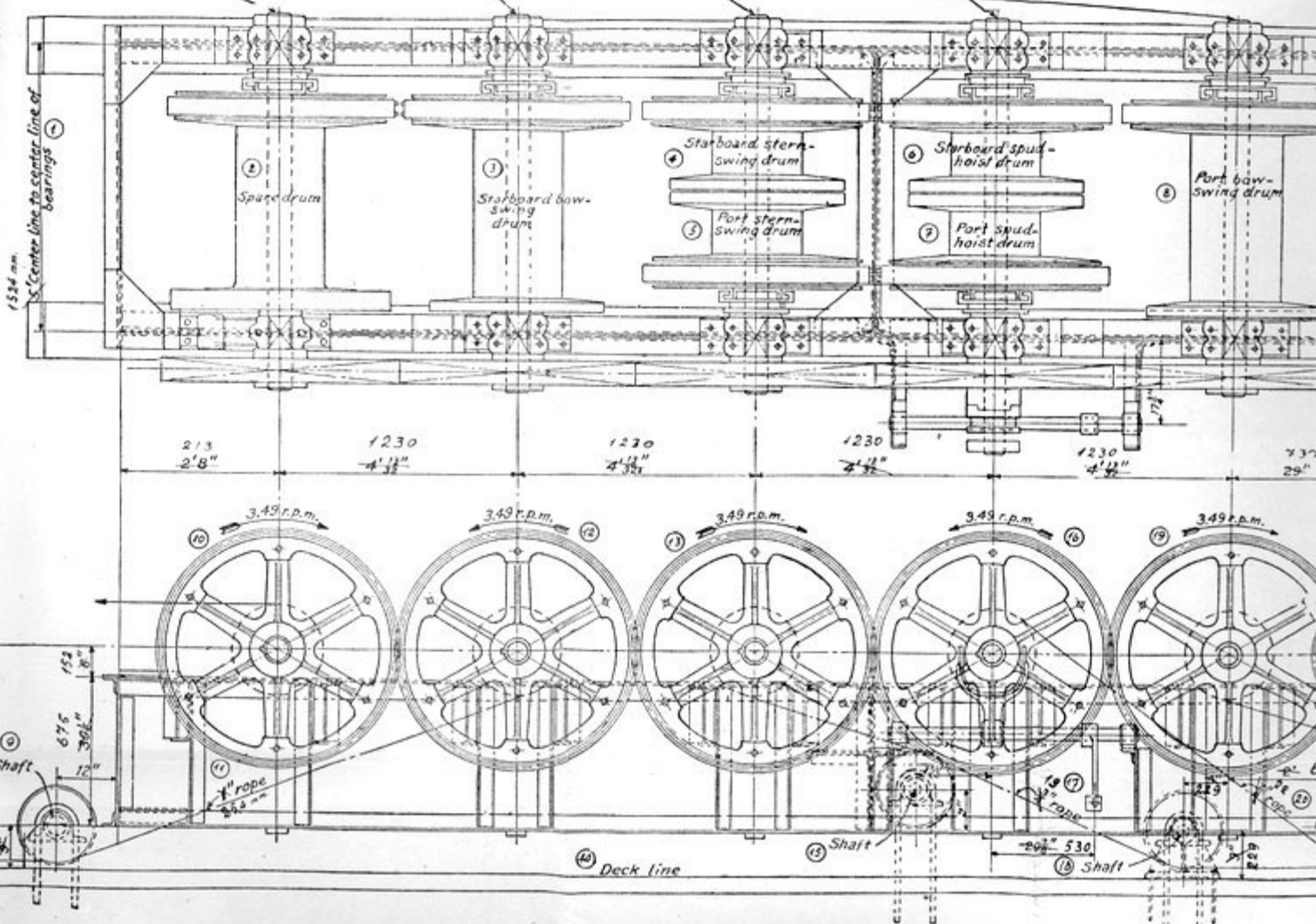
GENERAL ARRANGEMENT OF WINCHES ON A 9-FOOT DREDGE.
